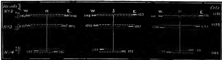
Levels of the "roads" transverse to the valley. 0 marks the level of the cols, and—that of the "roads."
